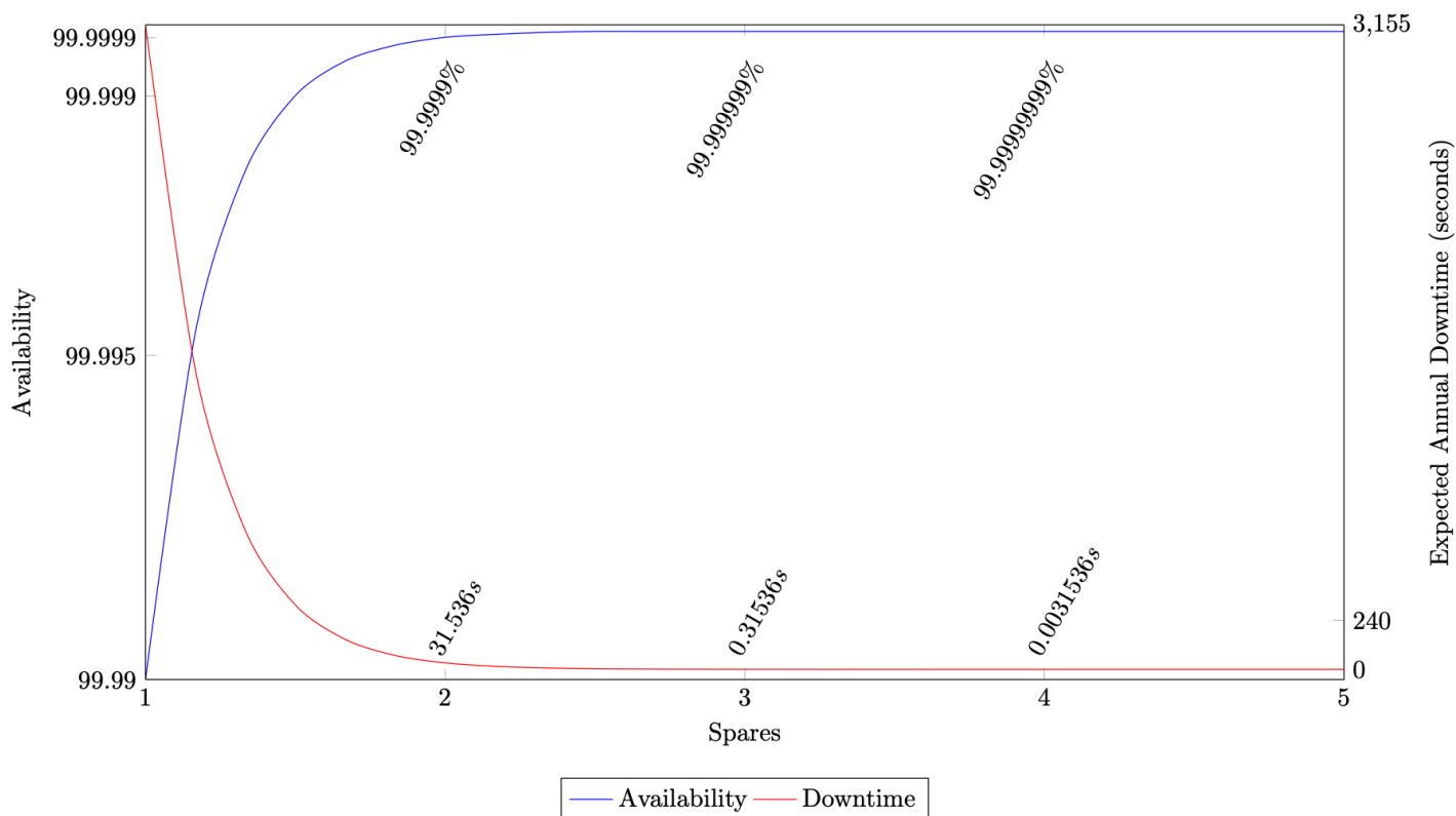
Effect of Sparing on Availability and Downtime
