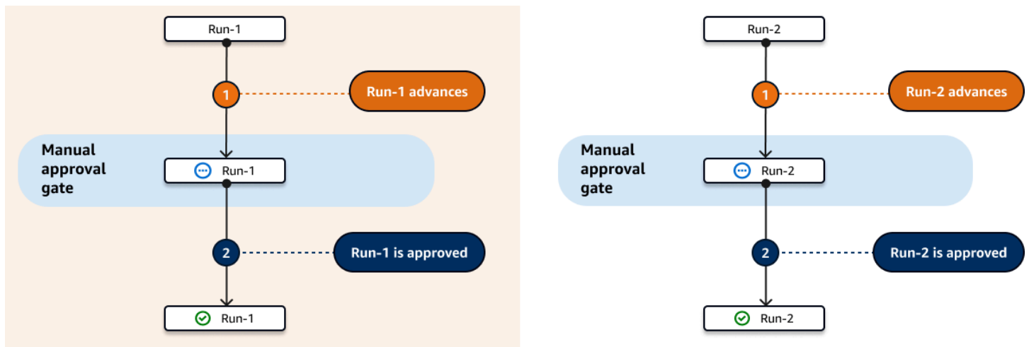
Figure 3: 'Parallel run mode' and an Approval gate
