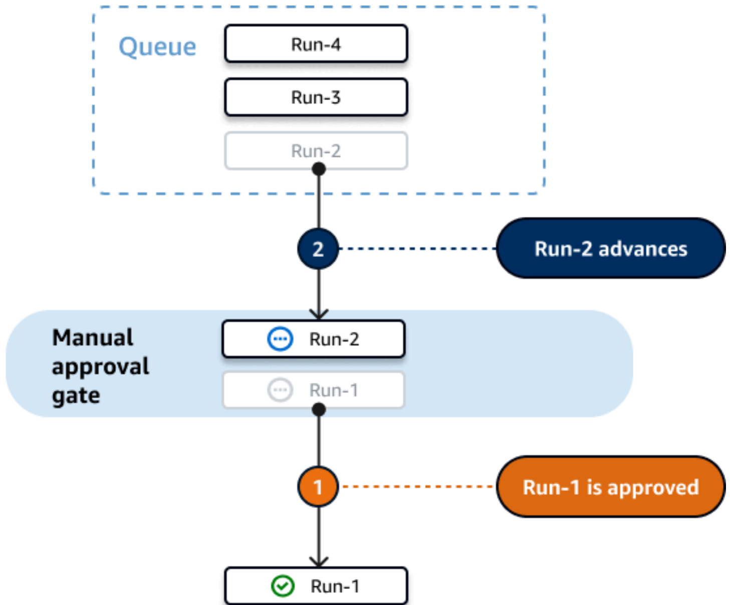
Figure 2: 'Superseded run mode' and an Approval gate
