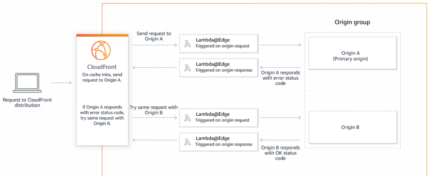
Figure 2 : Origin failover with Lambda@Edge functions triggered on origin request and response events.
