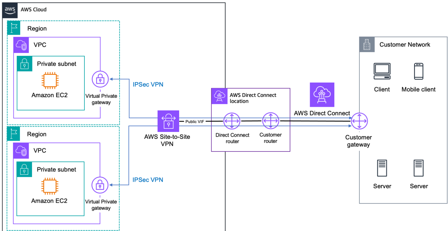
AWS Direct Connect and AWS Site-to-Site VPN
