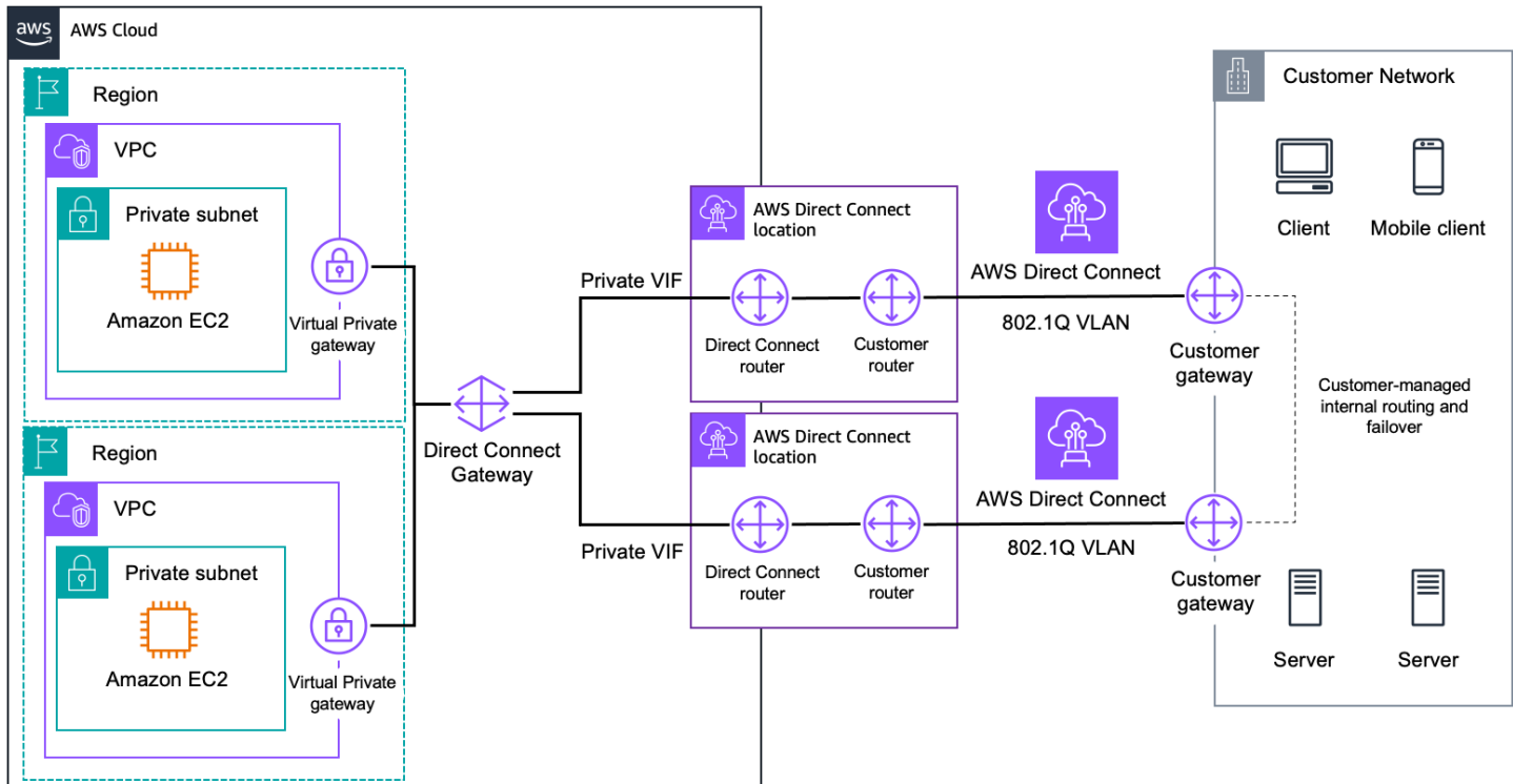
AWS Direct Connect Gateway
