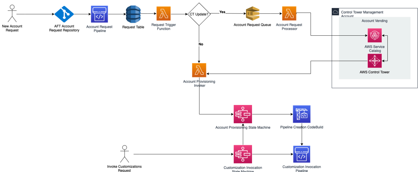
Figure 1: AWS Control Tower Account Factory for Terraform
